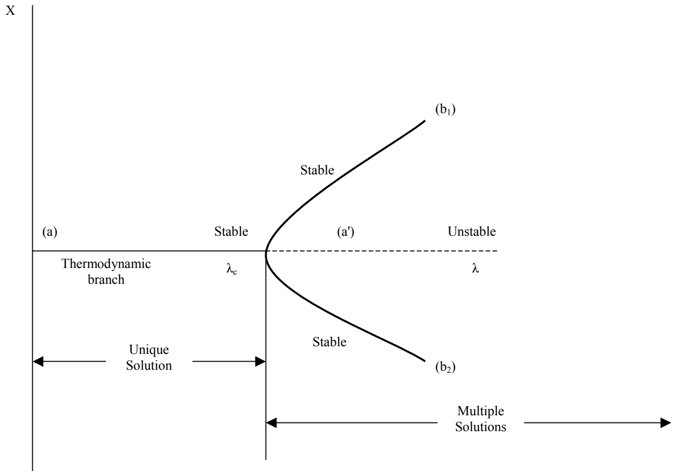
Figure 4 (from Nicolis & Prigogine, 1989, p72) Bifurcation diagram showing how a state variable X is affected when the control parameter \lambda varies. a unique solution ( a ), the thermodynamic branch, loses its stability at \lambda_c . At this value of the control parameter new branches of solutions ( b_1, b_2 ), which are stable at the example shown, are generated.
